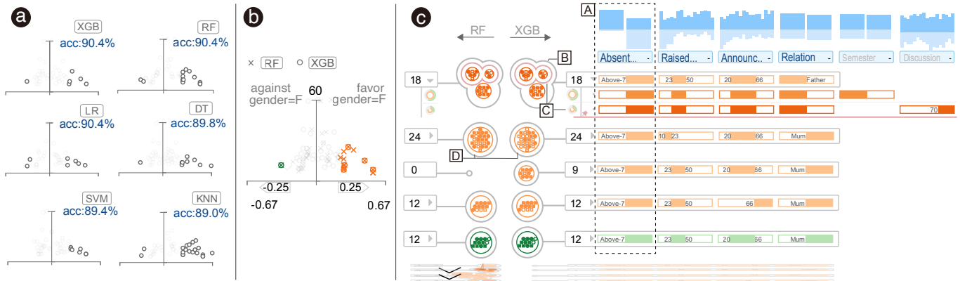
Fig. 12. Use DiscriLens to analyze discrimination: (a) analyze the discriminatory itemsets of different models using the scatter plots; (b) compare RF with XGBoost in a scatter plot; (c) compare RF with XGBoost in the comparison mode.
