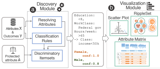
Fig. 4. DiscriLens consists of two main modules: a discovery module (a) and a visualization module (b).
