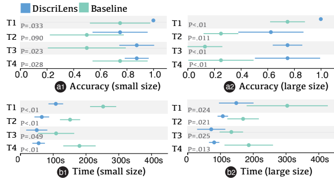
Fig. 10. Accuracy and completion time under different conditions. Error bars indicate 95% confidence intervals.
