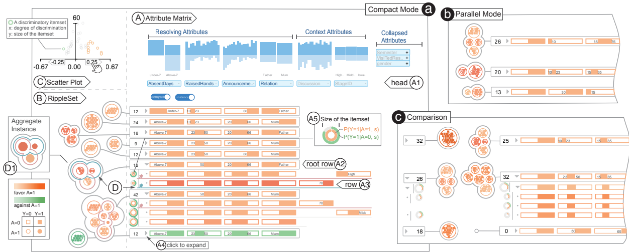
Fig. 6. The visual interface consists of three key components: the attribute matrix (A), the RippleSet (B), and the scatter plot (C). Three modes of analysis are supported: the compact mode (a), the parallel mode (b), and the comparison mode (c).
