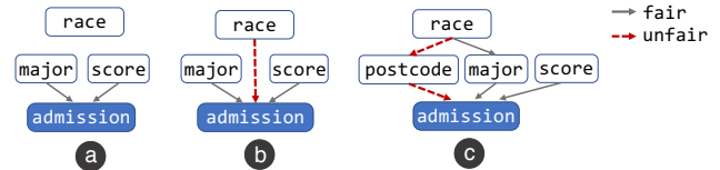
Fig. 3. In a toy example of college admission, different types of relationship exist between the protected attribute race and the result admission. (a) race doesn't influence admission. (b) race directly influences admission. (c) race indirectly influences admission through other attributes.
