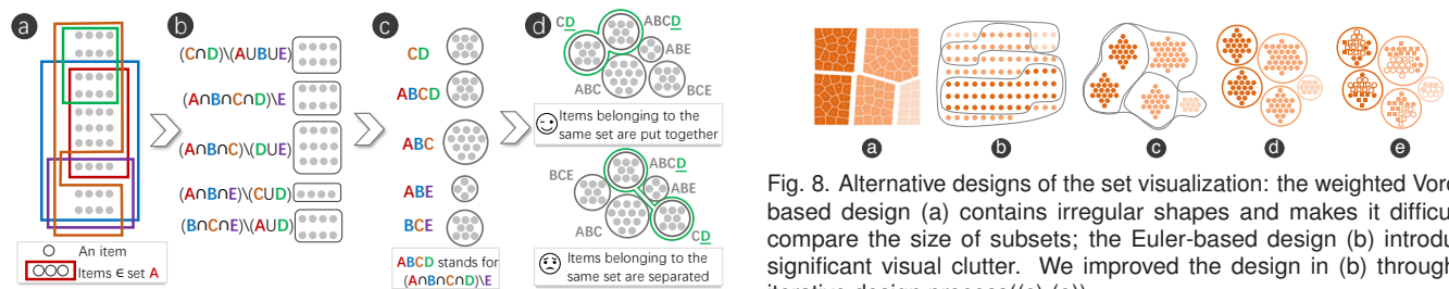
Fig. 7. RippleSet avoids the complex overlapping shapes in the traditional Euler diagram (a) by representing the maximal inseparable subset (b) as circles (c). Subsets belonging to the same set are put adjacent to one another to better present the composition of one set (d).
